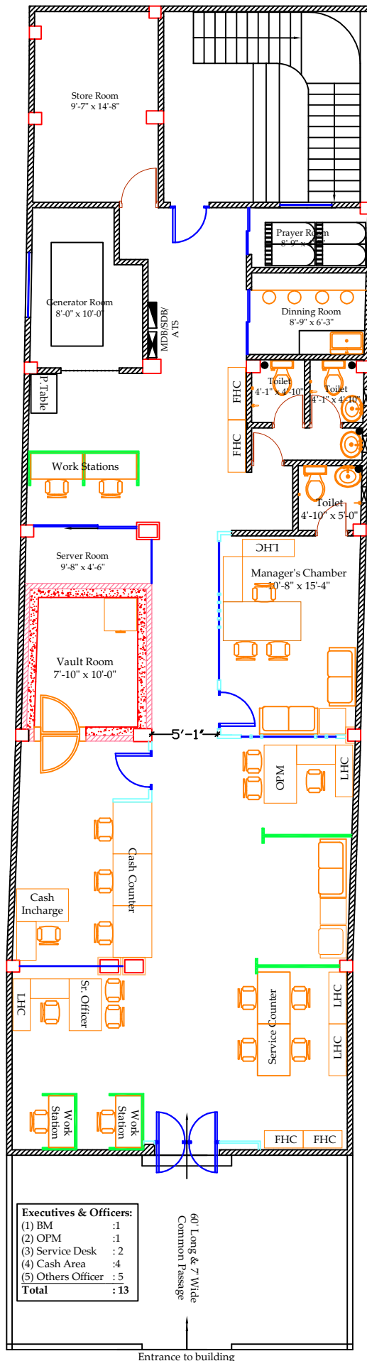
Furniture Layout Plan (Option-2) Proposed Abdullapur Branch, SBAC Bank Ltd
